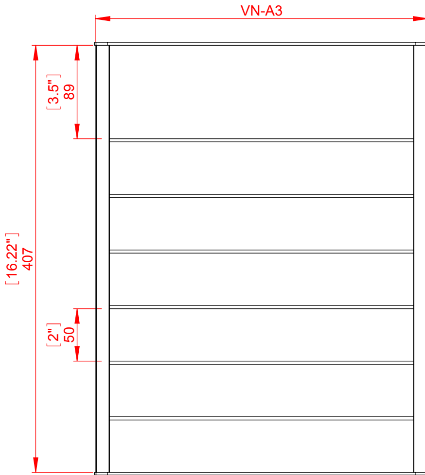
Front view
